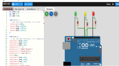
Figure 3. Wokwi Simulator Display During the Simulation Process
