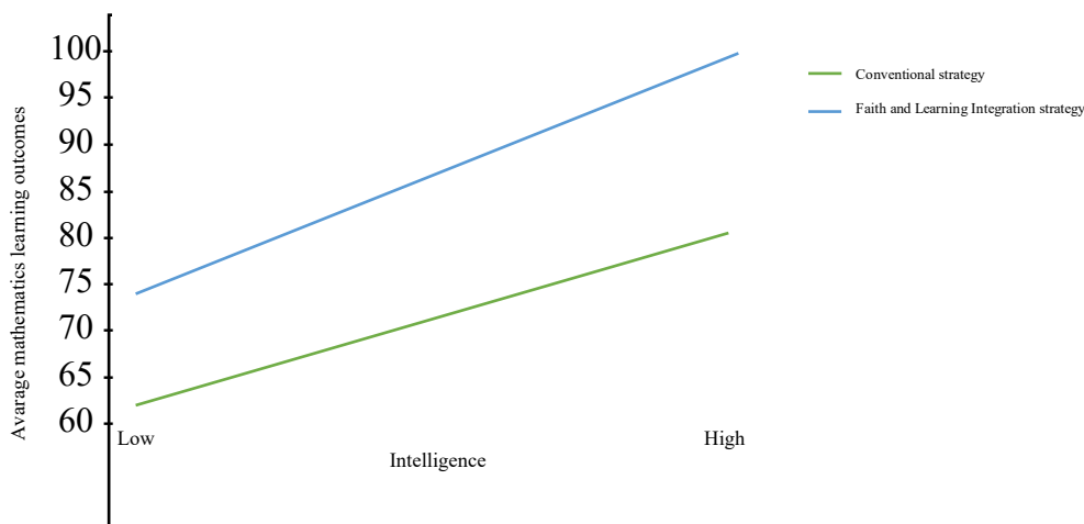
Figure 1. Interaction graph between instructional strategies and intelligence levels on students' mathematics learning outcomes.
